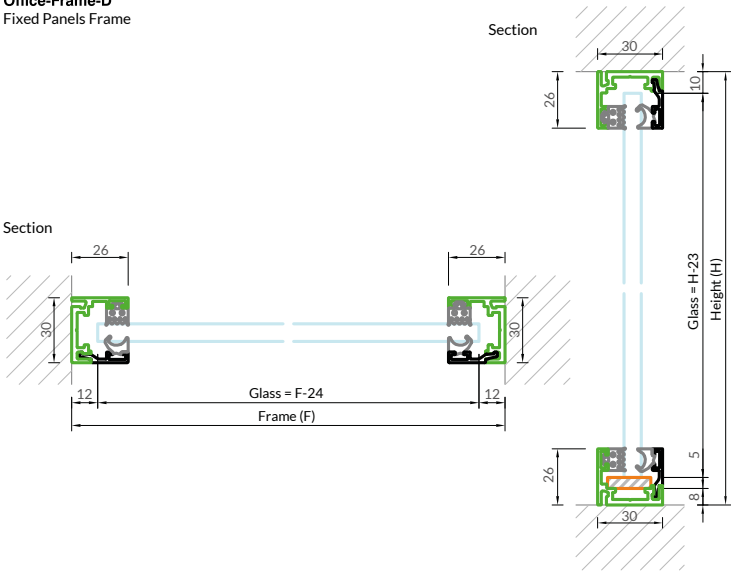
Office-Frame-D Fixed Panels Frame
